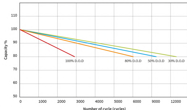
Cycle life with D.O.D at 25°C, 0.5C
